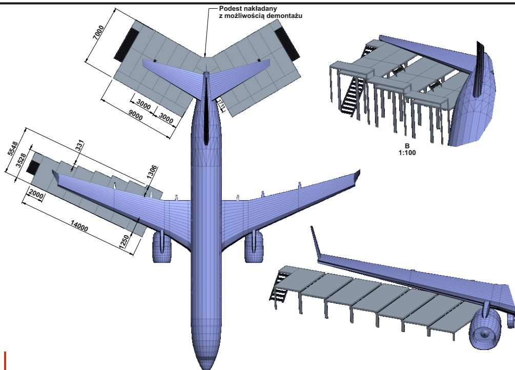
MOBILE SERVICE PLATFORMS DESIGNED FOR THE SIDE WINGS OF THE BOEING 737
