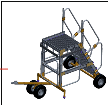
TOWABLE AIRCRAFT BOARDING STAIRS
