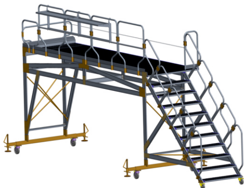
MOBILE SIDE PLATFORM
